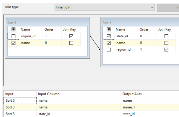
Fig. 9. Merge Join Transformation Editor
